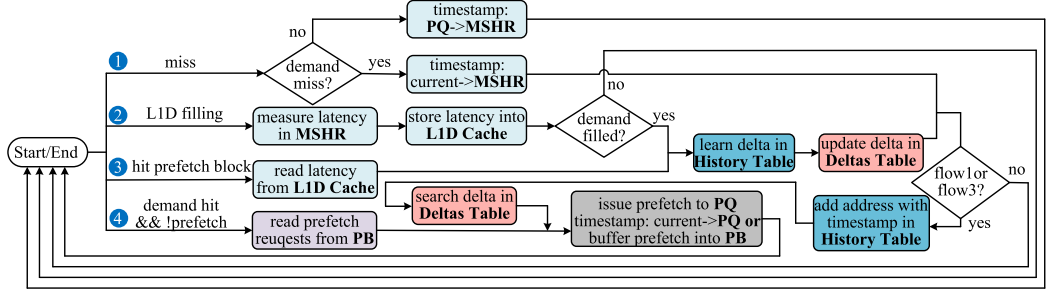
Fig. 5. Four working flows of Hyperion. Operations associated with the timeliness-aware delta training mechanism are represented by light blue blocks, while dark blue blocks denote operations within the History Table. The pink blocks signify operations in the Delta Table, while the gray block pertains to both the issuing mechanism and the timeliness-aware delta training mechanism. Finally, the purple block corresponds to the read operation of the prefetch buffer (PB).
